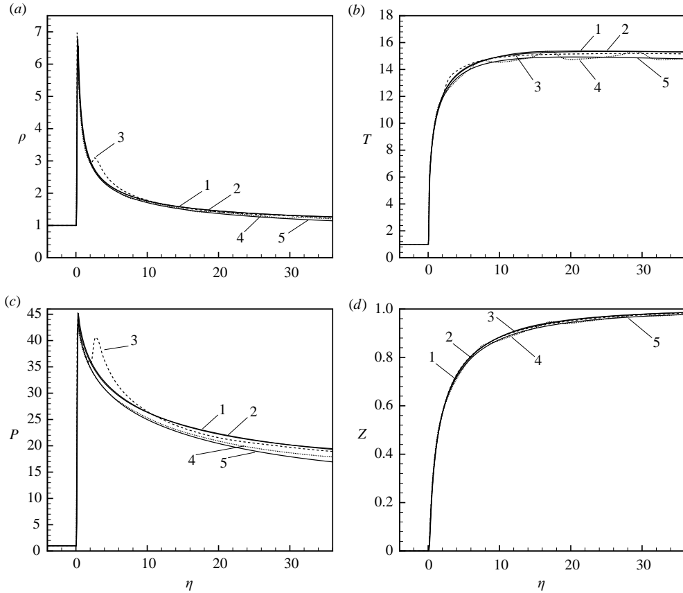
FIGURE 8. (a) Density, (b) temperature, (c) pressure and (d) progress variable profiles for 5 data sets extracted at t = 35.79 . Slices 1 and 5 are extracted along the plane of symmetry and the corner wall, respectively. The remaining data are taken in the shock normal direction and are evenly spaced along the detonation front.
