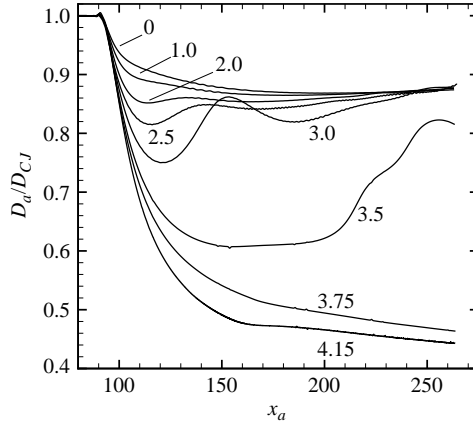
FIGURE 4. Detonation velocity at the plane of symmetry, D_a , as a function of the distance measured from the vertex, x_a . The labels are values of the reduced activation energy \theta_{CJ} , varying from 0 to 4.15.
