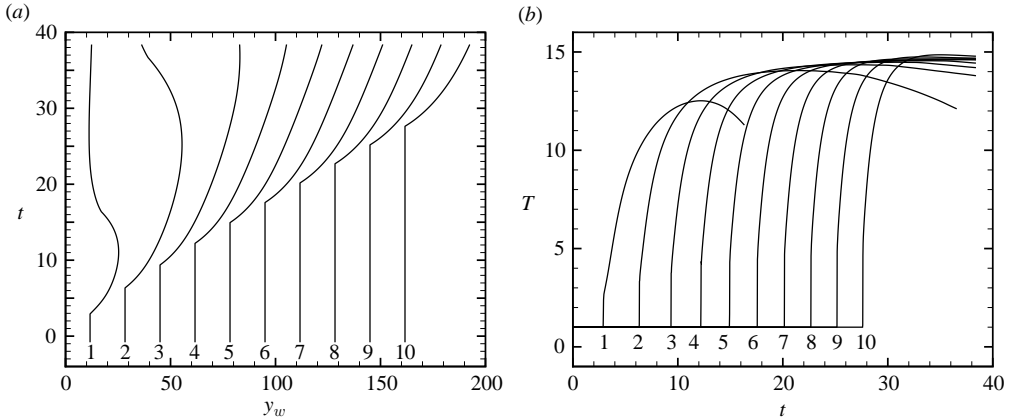
FIGURE 10. (a) Particle paths for 10 sample particles injected along the vertical corner wall for \theta_{CJ} = 1 . (b) Temperature profiles along the particle paths.
