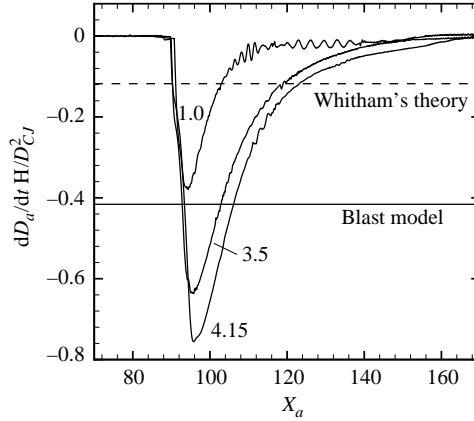
FIGURE 21. Shock deceleration as a function of the distance from the corner vertex, parameterized by \theta_{CJ} .
