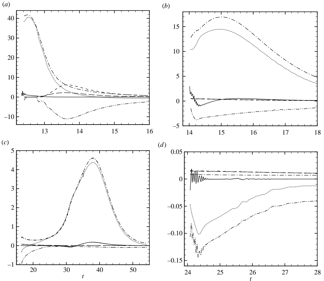
FIGURE 14. Terms in the reaction zone temperature (2.13) along the same particle paths as in figure 13 for \theta_{CJ}=4.15 . The particles are injected on the channel plane of symmetry. \cdots , Lagrangian temperature; - - - , heat release; - - - , curvature; - - - , transverse divergence; - \cdot - \cdot , unsteadiness. The solid line is the difference between the left-hand side and the right-hand side in (2.13), as computed from the terms above. (a) Particle 1; (b) Particle 3; (c) Particle 5; (d) Particle 10.
