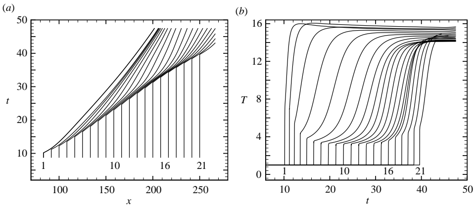
FIGURE 18. (a) Particle paths for 21 sample particles injected along the channel plane of symmetry (figure 9b) for \theta_{CJ} = 3.5 . The labels 1, 10, 16, 21 indicate particles that are analysed in terms of numerical dominant balance. (b) Temperature profiles along the particle paths.
