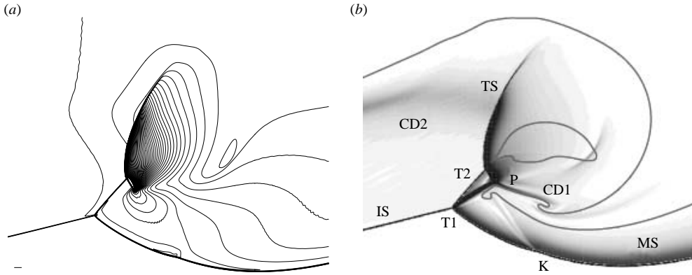
FIGURE 17. Structure of the re-ignition transverse wave: (a) contours of pressure and (b) numerical schlieren of density, at time t = 28.47 . In (a), the contour lines are spaced by the non-dimensional value 2.083 with a cutoff limit of 250 marking the pressure peak (at 445) behind the kink. The segment at the bottom left shows the length \Delta_{1/2} in the plot scale. The solid line in (b) is the 95% reaction completion locus.
