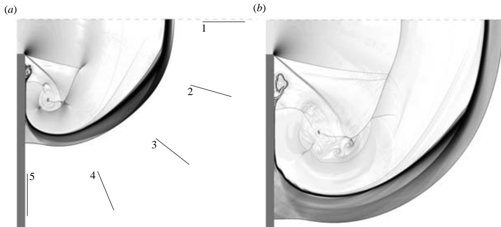
FIGURE 11. Numerical schlieren images for the case \theta_{CJ} = 4.15 at (a) t = 28.43 ; (b) 53.22 .
