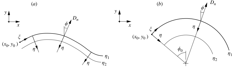
FIGURE 3. (a) Intrinsic coordinates \xi and \eta for an arbitrary front, and (b) specialized to a cylindrical front.
