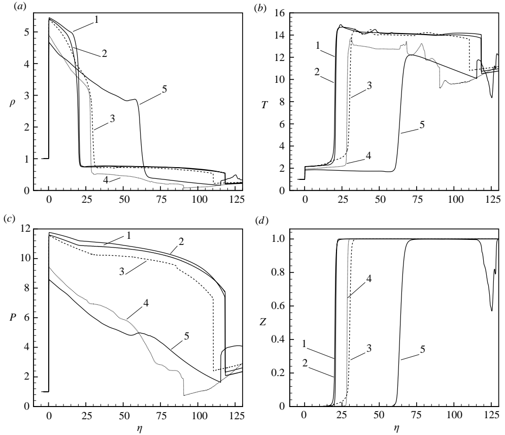
FIGURE 12. (a) Density, (b) temperature, (c) pressure and (d) progress variable profiles for 5 data sets extracted at t = 53.22 .
