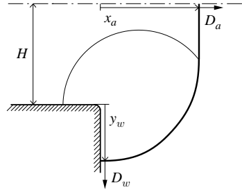
FIGURE 2. Detonation diffraction around a corner. ---, the plane of symmetry of the channel; H , the channel half-width. Also shown are the distances measured along the plane of symmetry, x_a , and along the corner wall, y_w .
