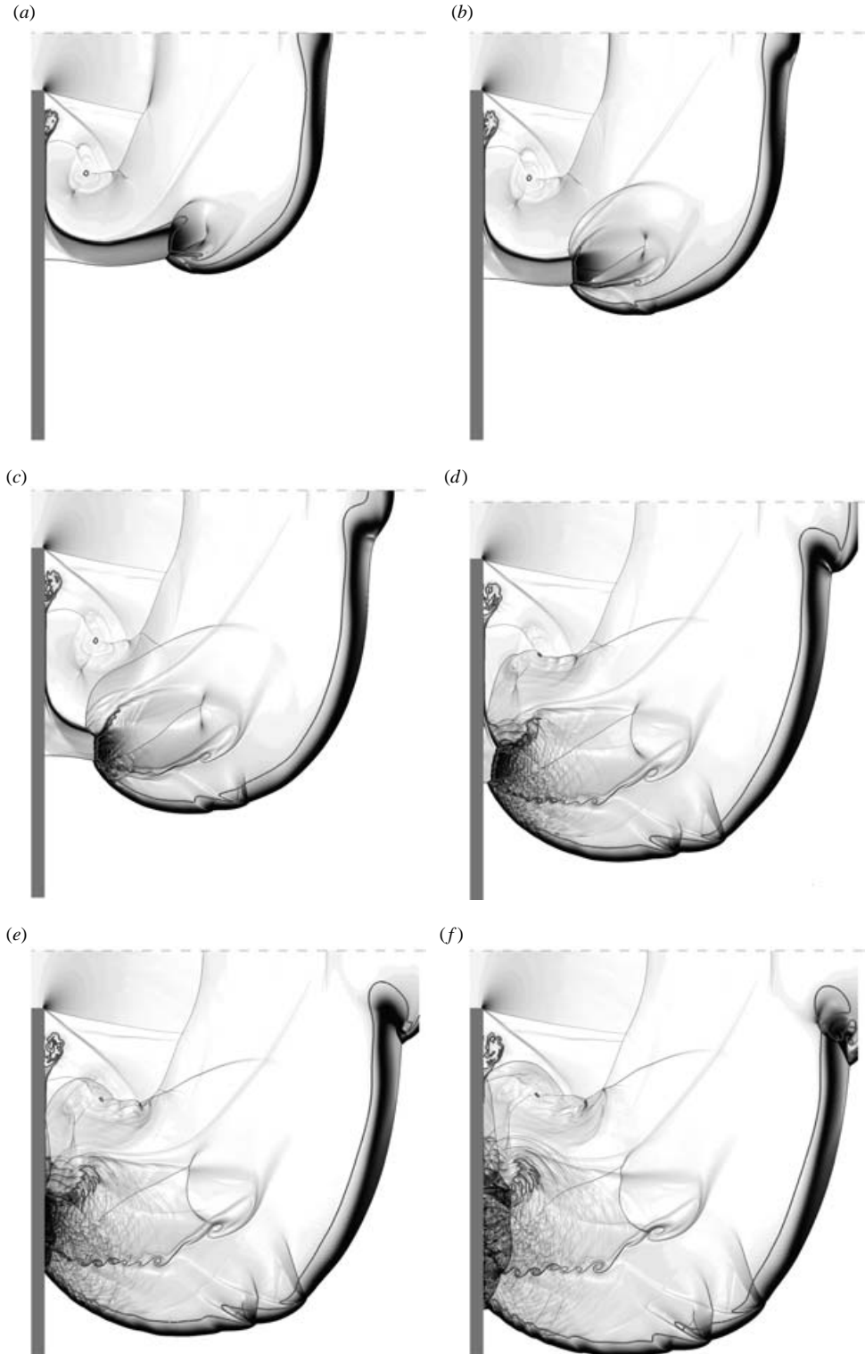
FIGURE 16. Numerical schlieren images for the case \theta_{CJ} = 3.5 . (a) 32.13; (b) 35.79; (c) 39.45; (d) 43.11; (e) 44.94; (f) 46.77.
