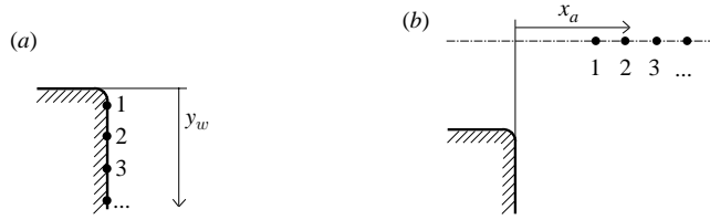
FIGURE 9. (a) Initial location of injected particles along the corner wall and the (b) plane of symmetry.
