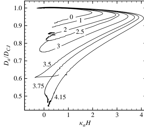
FIGURE 6. Detonation velocity–curvature ( D_n – \kappa ) diagram at the plane of symmetry of the channel. The labels are values of the reduced activation energy \theta_{CJ} , varying from 0 to 4.15.
