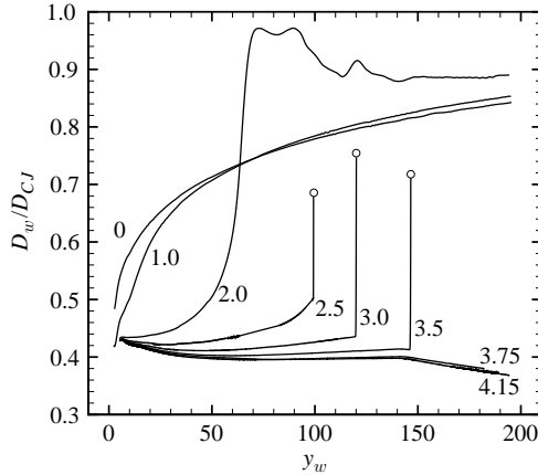
FIGURE 5. Detonation velocity at the corner wall, D_w , as a function of the distance from the vertex, y_w . The labels are values of the reduced activation energy \theta_{CJ} , varying from 0 to 4.15.
