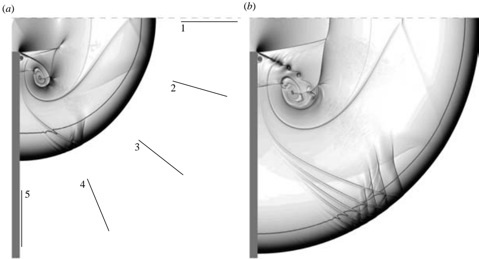
FIGURE 7. Numerical schlieren images for the case \theta_{CJ} = 1 . (a) t = 21.15 ; (b) 35.79. The solid line is the locus of 95% product.
