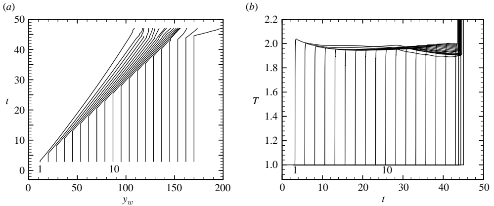
FIGURE 19. (a) Particle paths for 20 sample particles injected along the vertical corner wall (figure 9a) for \theta_{CJ} = 3.5 . The labels 1 and 10 indicate the particles that are analysed in terms of numerical dominant balance. (b) Temperature profiles along particles paths.
