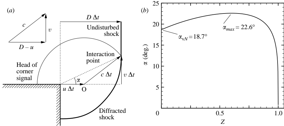
FIGURE 1. (a) Schematic of a diffracting shock (Skews' construction) in non-reactive gas. (b) Disturbance angle plotted vs. progress variable Z for a ZND-CJ detonation. Z=0 corresponds to post-shock conditions, Z=1 corresponds to the end of the reaction zone.
