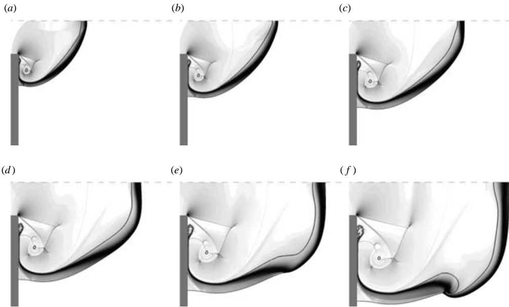
FIGURE 15. Numerical schlieren images for the case \theta_{CJ}=3.5 . (a) 10.17; (b) 13.83; (c) 17.49; (d) 21.15; (e) 24.81; (f) 28.47. The solid line is the locus of 95% product.
