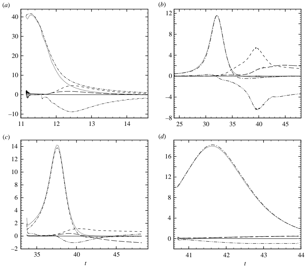
FIGURE 20. Terms in the reaction zone temperature (2.13) along the same particle paths as in figure 18(a) for the case \theta_{CJ} = 3.5 . The particles are injected along the plane of symmetry. \dots , Lagrangian temperature; -\cdot- , heat release; --- , curvature; --- , transverse divergence; --- , unsteadiness. The solid line is the difference between the left-hand side and the right-hand side in (2.13), as computed from the terms above. (a) Particle 1; (b) Particle 10; (c) Particle 16; (d) Particle 21.
