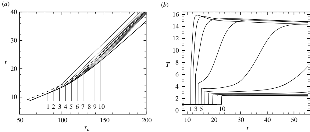
FIGURE 13. (a) Particle paths for ten sample particles on the plane of symmetry. Shock (thick solid line); traces of 5% and 95% of reaction completion (dashed lines); particle paths (thin solid lines). (b) Temperature profiles along the particles paths.
